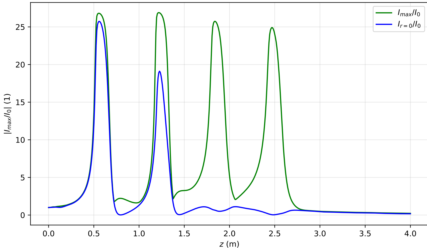
I_{max}(x=0, y=0, z)/I_0 , \text{Pin}=4.1\text{Pcr} , noisy input, artificial time
